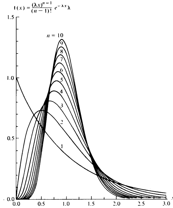
Figure 2.3. Graphs of the Erlangian density function of order n , for n = 1, 2, \dots, 10 . The densities have been normalized to have mean unity by taking \lambda = n . Adapted from L. Kosten, Stochastic Theory of Service Systems , New York: Pergamon Press, 1973.
